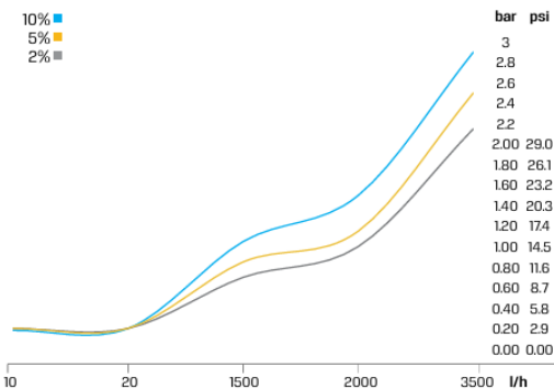
Pressure Loss
